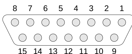
Figure 1.6 DIAGNOSTIC INTERFACE WIRING ON THE COMPRESSOR UNIT
