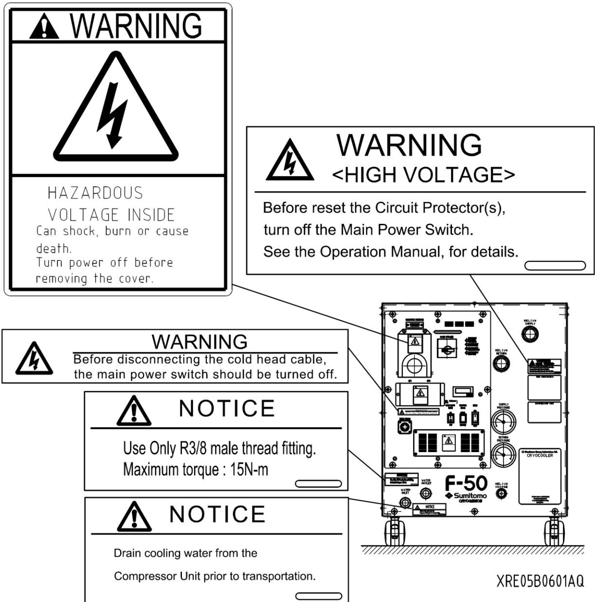
Figure 1.7 HAZARD ALERT LABEL LOCATION
